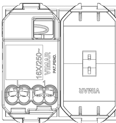
09001 - 1P 16AX 1-way switch white
